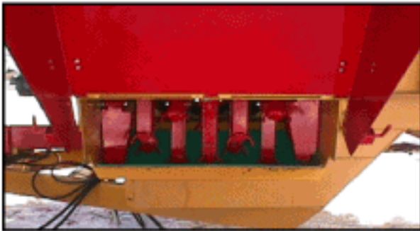
VIEW OF FLAILS AND AIR BOOSTER BLADES
