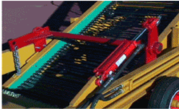
HYDRAULIC STEERING RUNNING GEAR IS CONTROLLED FROM THE TRACTOR FOR A CLOSER TURNING RADIUS OR RUNNING ALIGNMENT.
