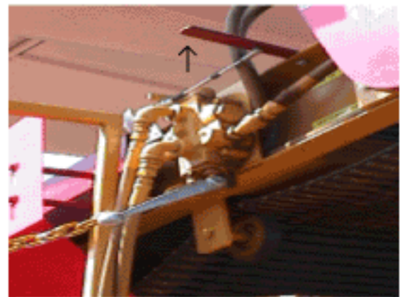
REMOTE START/STOP SORTING CONVEYER CONTROL LEVERS ARE LOCATED AT EACH END OF THE SORTING TABLE.
