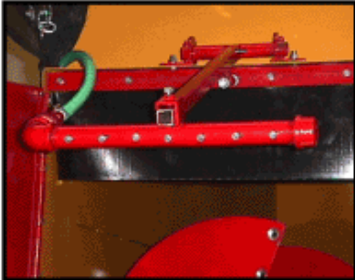
HINGED & ADJUSTABLE SPRAY BAR IS DESIGNED TO PUT OUT AN EVENLY DISTRIBUTED SHEET OF MOLASSES. THIS PIPE IS SLOTTED THE FULL LENGTH & IS ADJUSTED ONCE BY THE BOLTS ALONG THE SPRAY BAR, AND SET TO THE VISCOSITY OF THE MOLASSES. EASILY CLEAN BY RUNNING BLADE IN THE SLOT THE FULL LENGTH.
