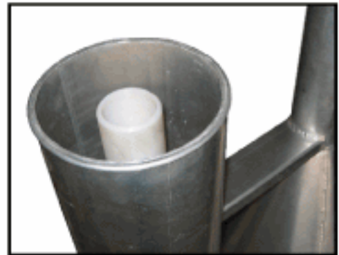
WASTE WATER DISCHARGE HAS AN ADJUSTABLE THREADED SLEEVE THAT CONTROLS THE WATER LEVEL IN SIGHT GAUGE, ONCE ADJUSTED PROPERLY WILL AUTOMATICALLY KEEP WATER FROM DISCHARGING THROUGH OIL OUTLET.
